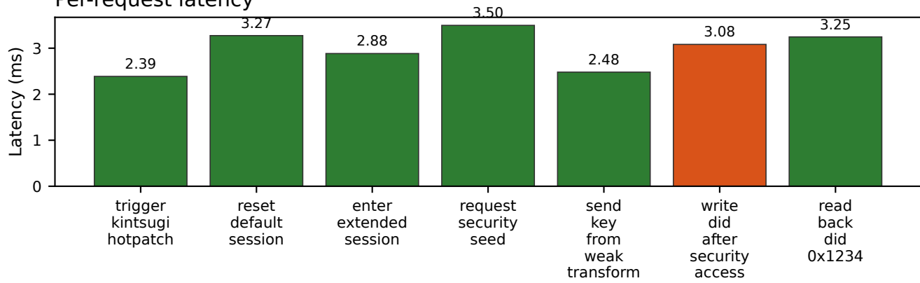
Per-request latency
