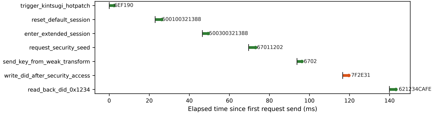
Per-request latency
